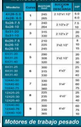
1750 RPM
