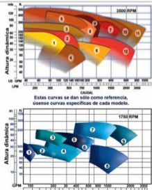
1750 RPM
